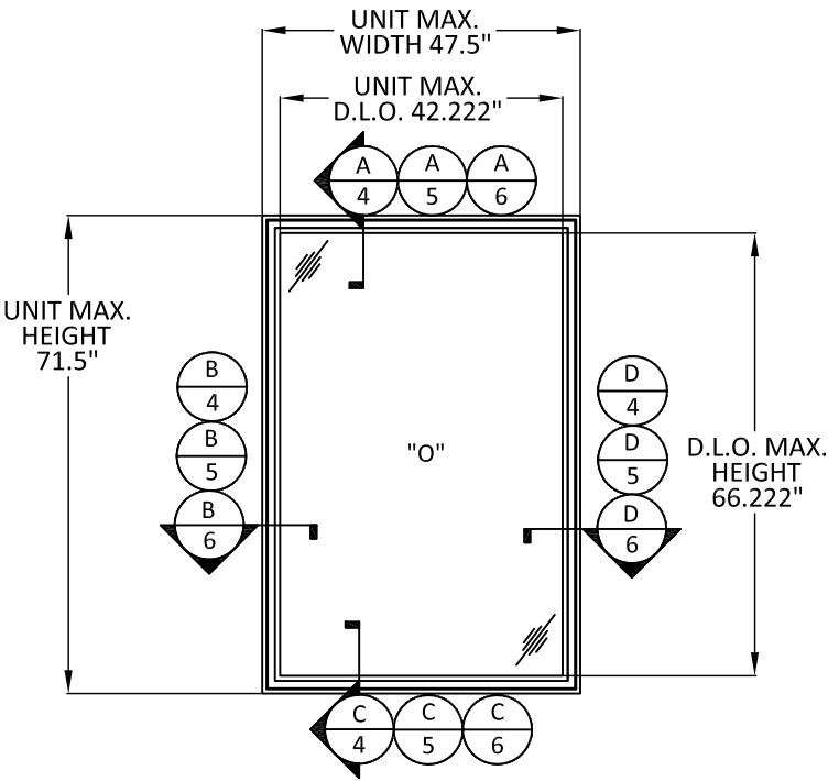
TYPICAL ELEVATION CASEMENT FIXED WINDOW
