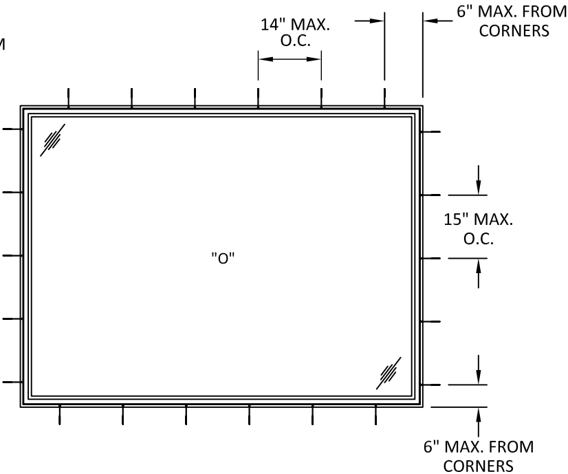
TYPICAL ANCHOR LAYOUT THROUGH FRAME INSTALLATION
