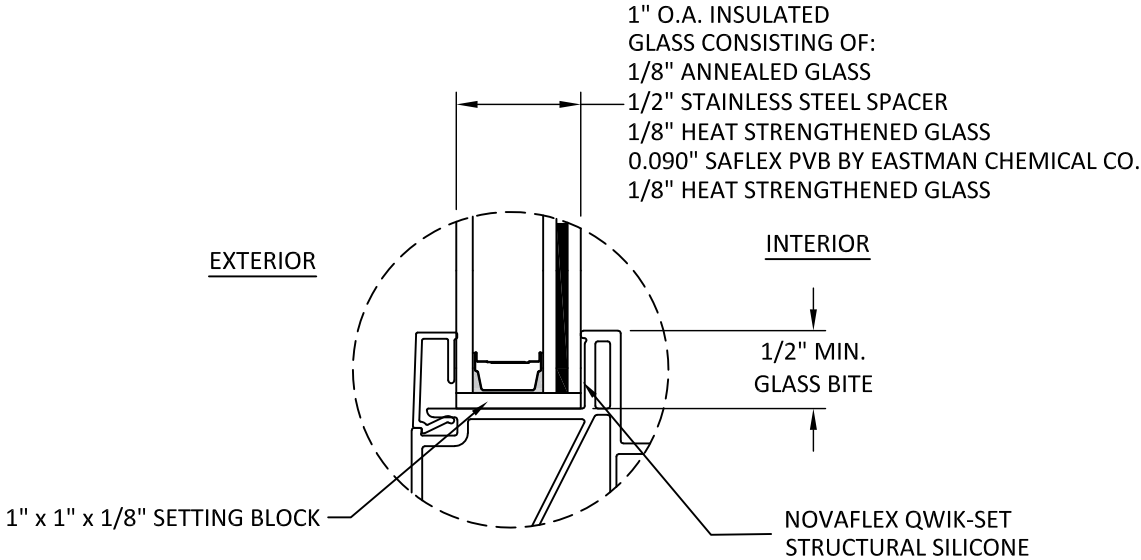
GLAZING DETAIL 2
