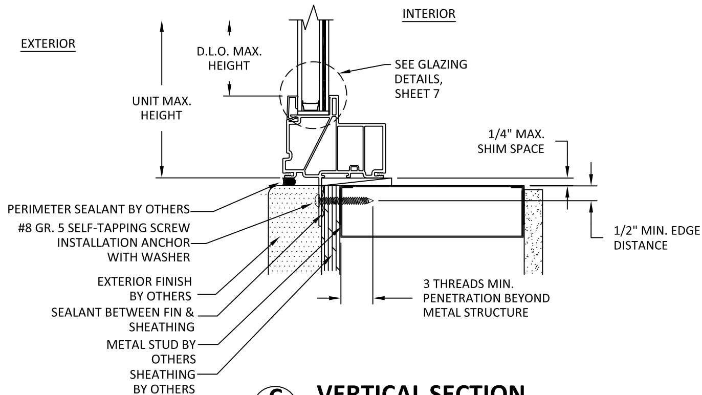
C 4 VERTICAL SECTION NAIL FIN INSTALLATION METAL SUBSTRATE
