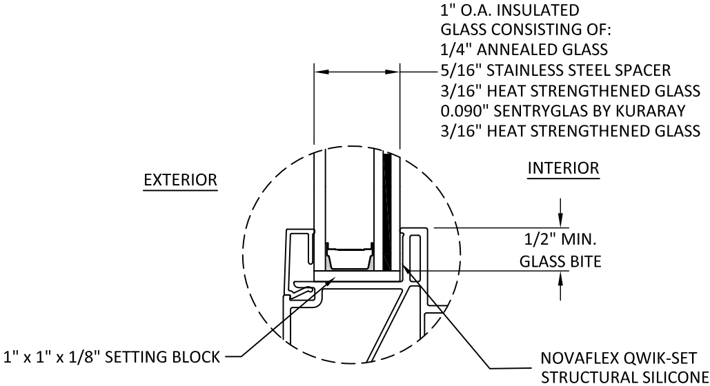
GLAZING DETAIL 1
