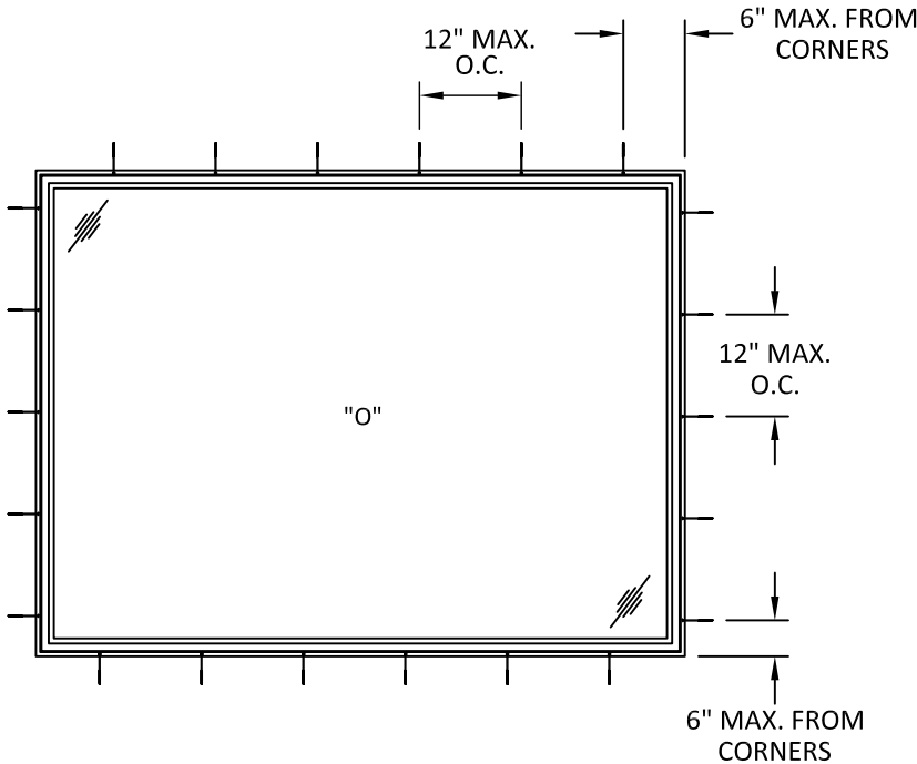
TYPICAL ANCHOR LAYOUT CLIP INSTALLATION
